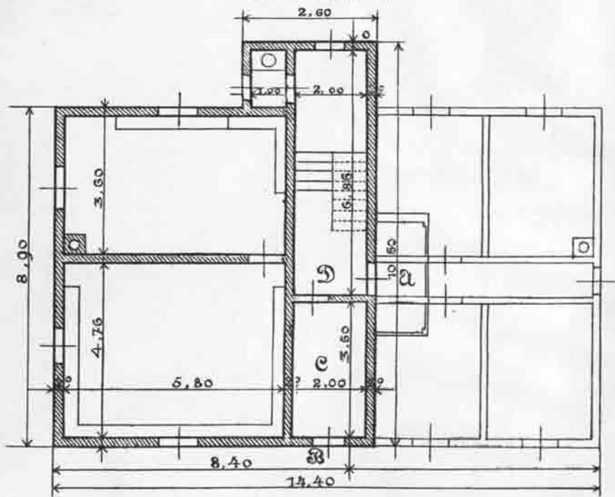
Erdgeschoss.
