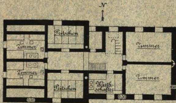
Dachstock.
