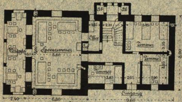
Erdgeschoss.
