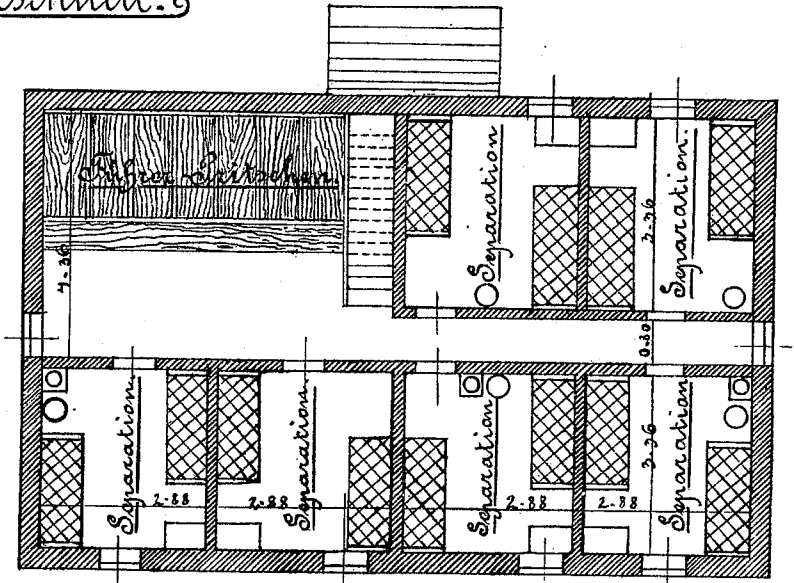
1. Stock.
