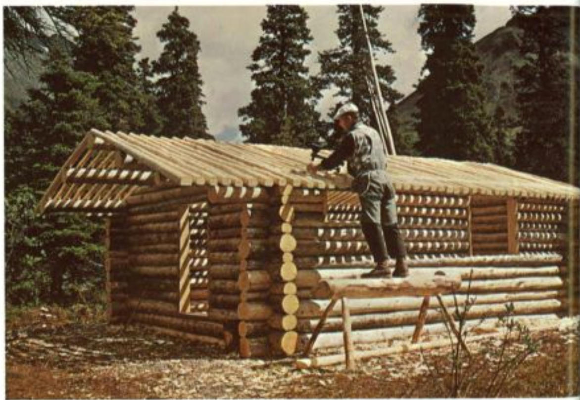
The roof poles were nailed at right angles to eave, purlin and ridge logs.
