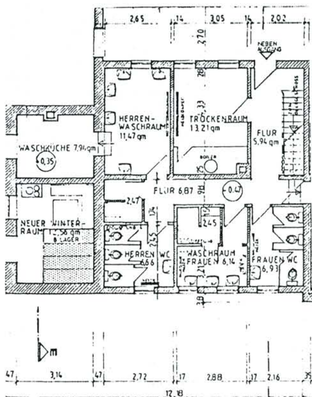
Grundriß Erdgeschoß
